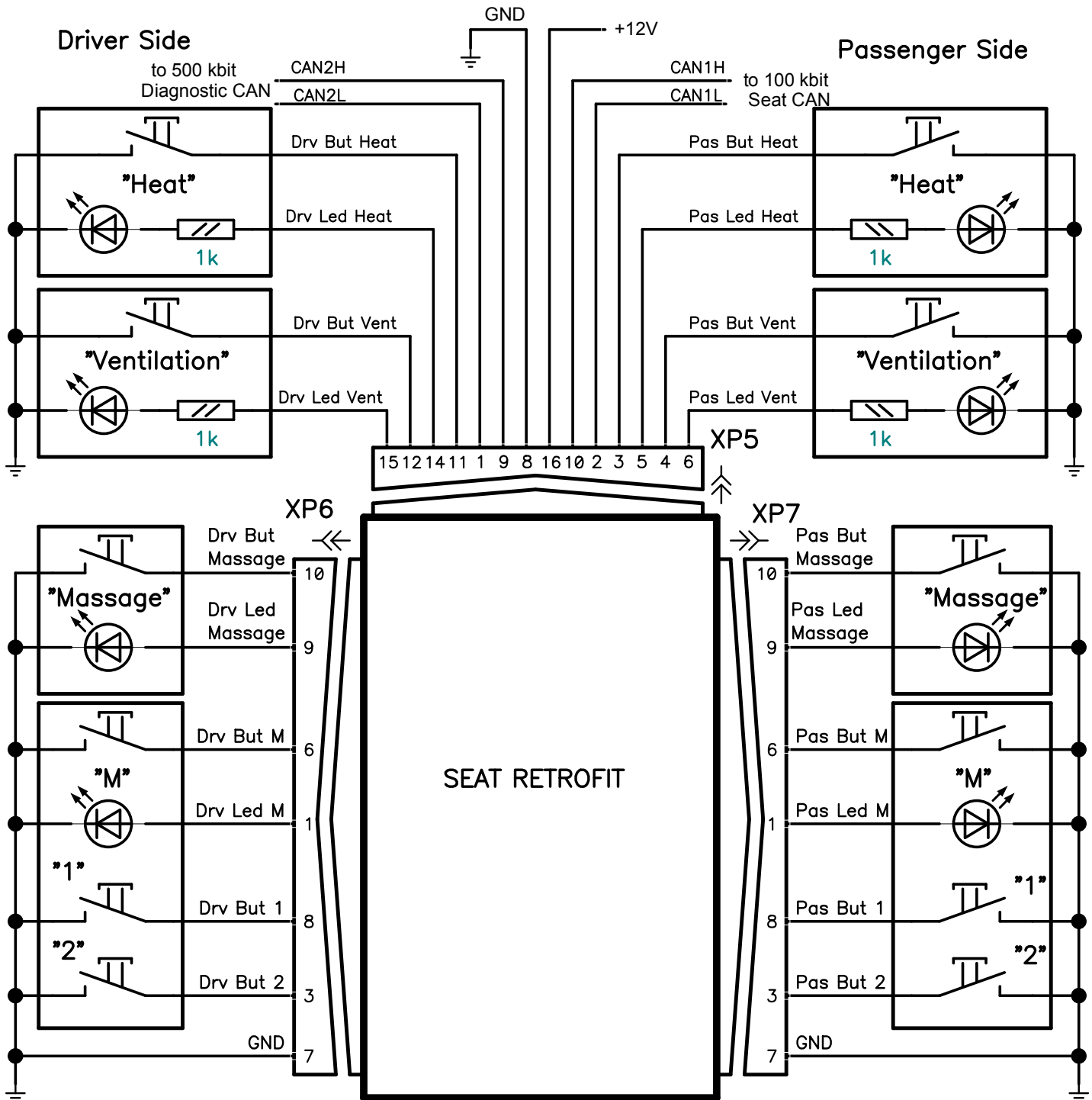
Fig 2. Module connection
