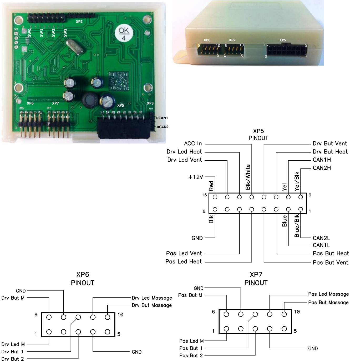
Fig 1. Module design and its pinout
