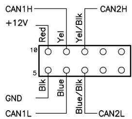
Fig 1 Design and pinout of the adapter
