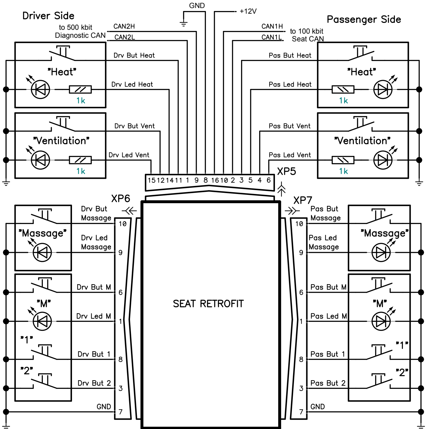
Fig 2. Module connection
